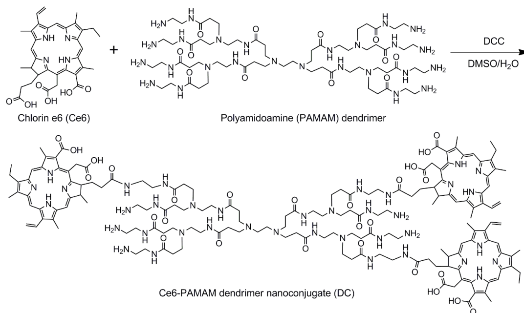
Figure 1. Schematic diagram of synthesis of hydrophilic Ce6-PAMAM dendrimer nanoconjugate (DC).
